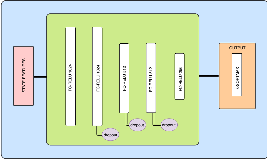
Fig. 1. Network architecture used across all game types for both soloist and defenders.
