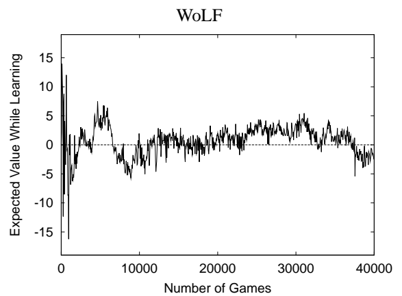
Figure 4: Expected value of the game while learning.
