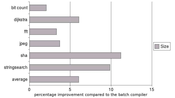
Figure 24: Size Only Improvements for the ARM
