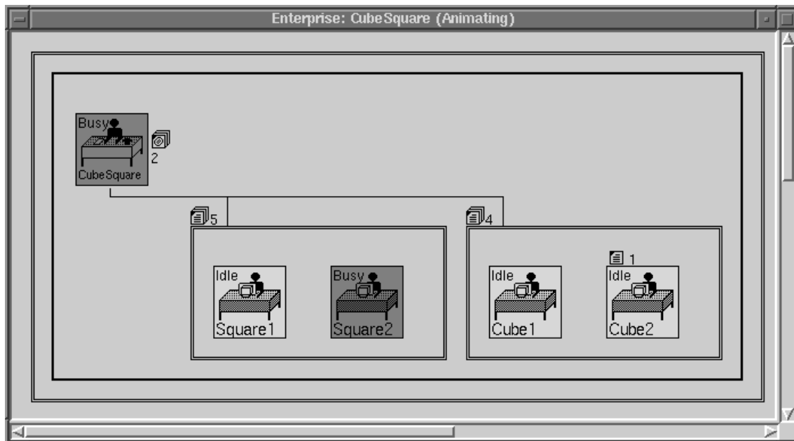
Figure 3. CubeSquare animating.
