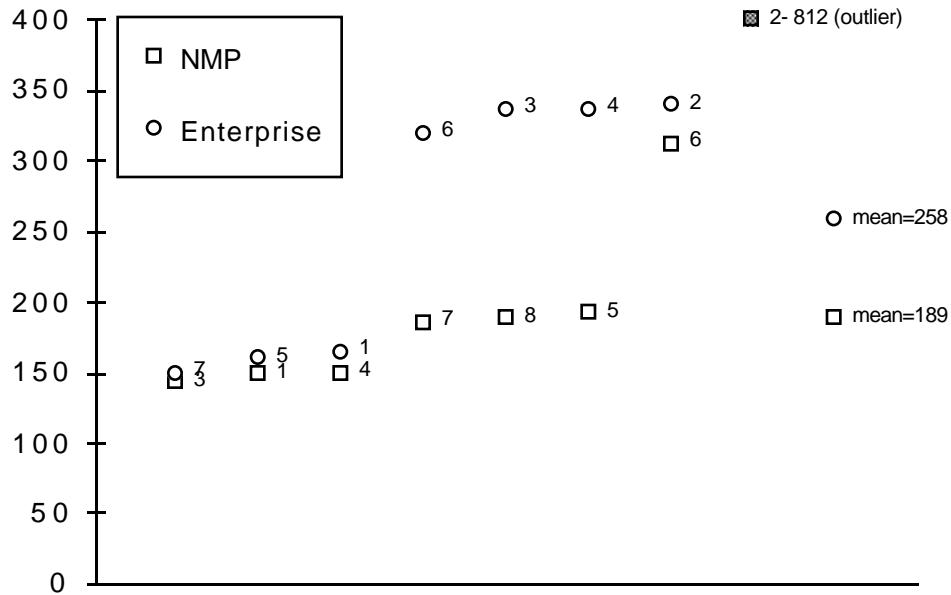
Figure 8. Parallel Performance in Seconds
