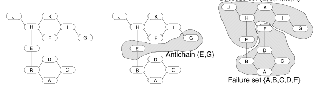
Figure 1: Antichains in partial order bounding
