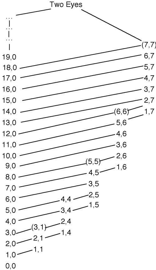
Figure 8: Partial order evaluation of (liberty, eye) pairs
