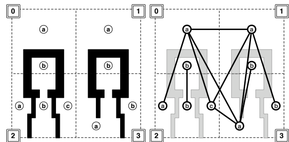
Figure 1: The abstraction used in Dragon Age: Origins.
