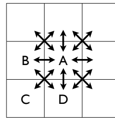
Figure 3: The possible edges which must be checked when adding the grid cell marked “A”.
