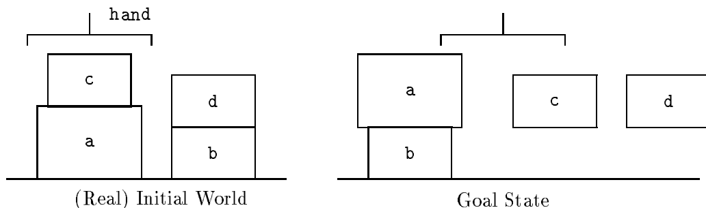
Figure 1: Blocks world: Initial and Goal configurations
