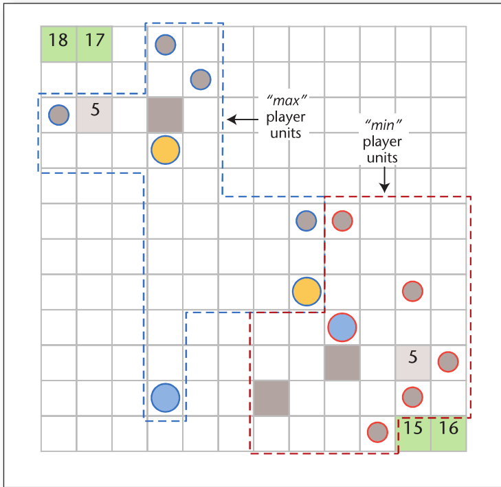
Figure 1. A Screenshot of the \mu RTS Simulator.
