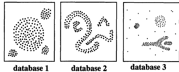
figure 1: Sample databases
