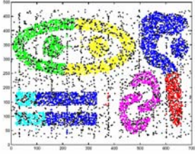
Figure 6: CURE's clustering result on t7.10k.dat with k = 9 , \alpha = 0.3 , and number_of_representative_points = 10
