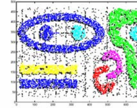
Figure 11: WaveCluster's clustering result on t7.10k.dat with resolution = 5 and \tau = 1.5
