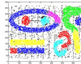
Figure 10: DBSCAN's clustering result on t7.10k.dat with \epsilon = 5.5 and MinPts = 1
