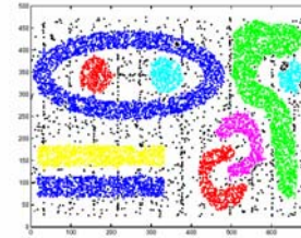
Figure 9: DBSCAN's clustering result on t7.10k.dat with \epsilon = 5.9 and MinPts = 1
