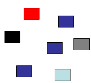
Labeling=Classification
